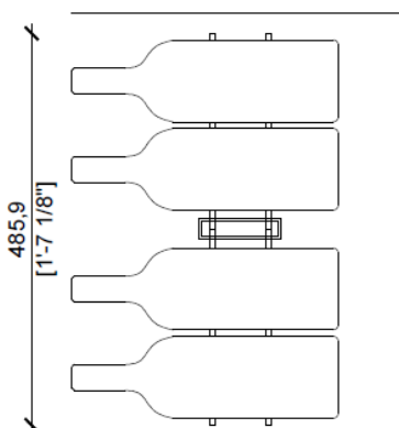
M2 - Magnum 2 Deep 2 Sides
