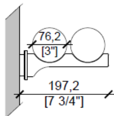
S2 - Standard 2 Bottle
