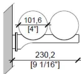
M2 - Magnum 2 Bottle
