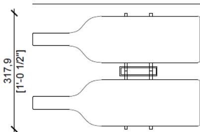
DM1 - Double Magnum 1 Deep 2 Sides
