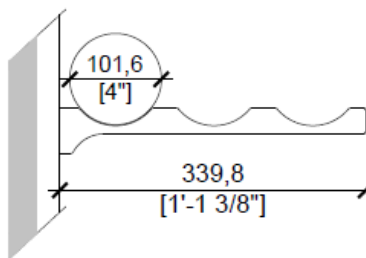
M3 - Magnum 3 Bottle
