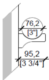
S1 - Standard 1 Bottle
