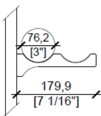
S2 - Standard 2 Bottle
