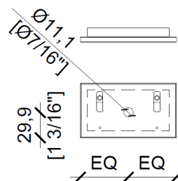
Mono plate detail with hole for light shelf wiring
