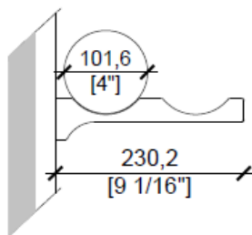
DM2 - Dbl Magnum 2 Bottle
