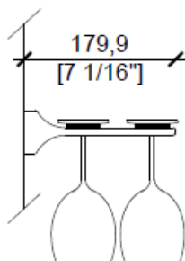
WG2 - Double Wine Glass Holder
