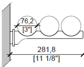
S3 - Standard 3 Bottle
