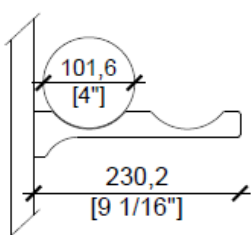
M2 - Magnum 2 Bottle
