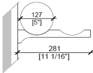
DM2 - Dbl Magnum 2 Bottle
