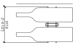
DOUBLE MAGNUM 1 DEEP (DM1) - 2 SIDES
