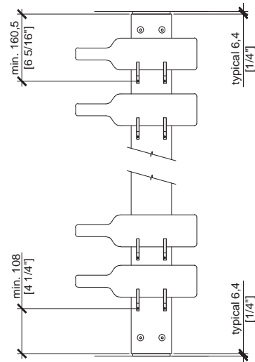
Post & Shoe Component
