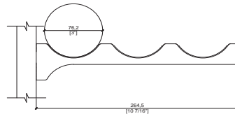
Standard - 3 Bottle (S3)
